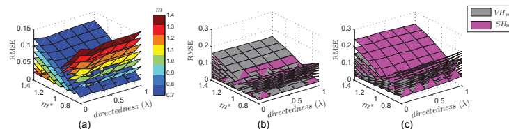
FIG 6. Sensitivity analysis of \hat{p}_A^{VH_m} and \hat{p}_A^{SH_m} on Net1 and Net2 with tested m values. (a) Net1, \hat{p}_A^{SH_m} not shown as it is similar to \hat{p}_A^{VH_m} ; (b) Net2 with homophily h_A = 0 ; (c) Net2 with homophily h_A = 0.4 . Each surface stands for simulation results with a fixed m value. Sampling without replacement, number of seeds=10, coupons=3, sample size=500.
